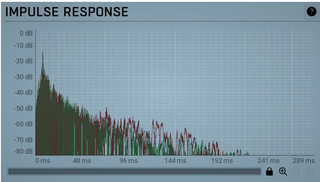
Impulse response
